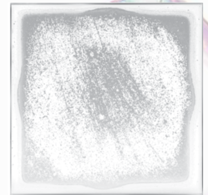
(C) UNCOATED CLEAR TEMPERED SHOWER GLASS Haze after testing 77%
